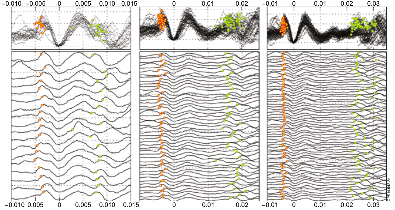
Figure 2: ELM occurrence times superimposed on VLD3 signal. Multiple time traces for different pairs of successive ELMs are displayed in three panels, corresponding to the first three groups of inter-ELM times indicated by red vertical lines in Fig.1. The three panels plot VLD3 signals (black dotted lines) for all ELMs for which the inter-ELM time interval is in the range: (left) \Delta t < 0.015 (centre) 0.015 < \Delta t < 0.025 (right) 0.025 < \Delta t < 0.035 . These traces have all been shifted in time such that t = 0 is at the first minimum in the VLD3 signal following the first ELM. Amplitude is set to zero at t = 0 . The VLD3 signal is normalized as in [6]. In the upper panels, the ELM times are marked on each VLD3 trace with yellow filled red circles (first ELM) and green circles (second ELM). The lower panels are a stack of the individual VLD3 signals, with ELM times denoted by red (first ELM) and green (second ELM) circles.
