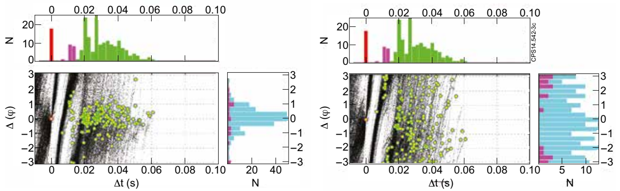
Figure 3: Left set of panels: ELM occurrence times and VLD3 phase difference between all pairs of ELMs in the flat-top of JET Pulse No: 83769. Right set of panels: same format as left panel, but with randomly shuffled time order of the inter-ELM time intervals. Each set of panels is as follows. Main panel: VLD3 instantaneous phase, modulo 2\pi , plotted as a function of time, up to the occurrence time of the next ELM. The coordinates are time, and phase difference from the occurrence time of the first ELM. ELM occurrence times are marked on each VLD3 trace with yellow filled red circles (first ELM) and green circles (second ELM). Right hand panel: histogram of VLD3 phase difference at the time of the second ELMs, for inter-ELM time intervals \Delta t < 0.015 (magenta) and for all ELMs (cyan). Top Panel: histogram of inter-ELM time intervals.
